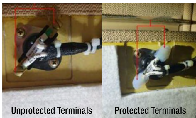
Figure 4-4. Following multiple injuries, exposed terminals (left side) are directed to be protected with an adhesive non-conducting sealant.
